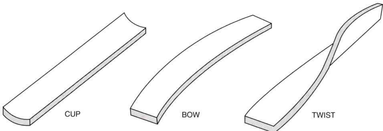
FIGURE 1: DRYING EFFECTS
